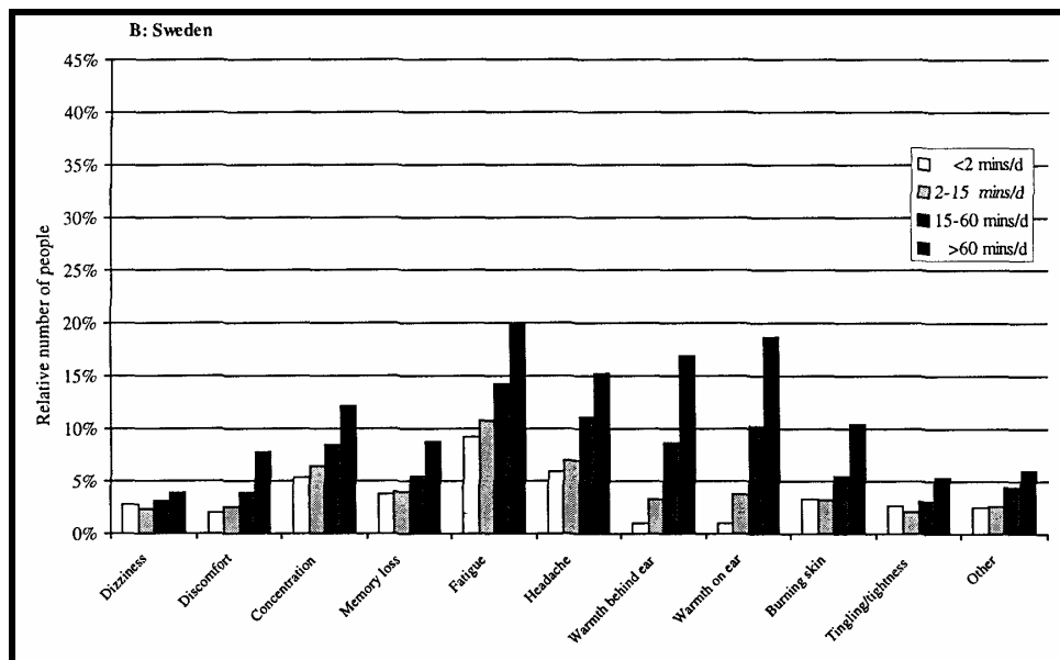
Figure 47: Prevalence of symptoms for Swedish mobile phone users, mainly digital, with various categories of length of calling time per day, Mild et al. (1998).
