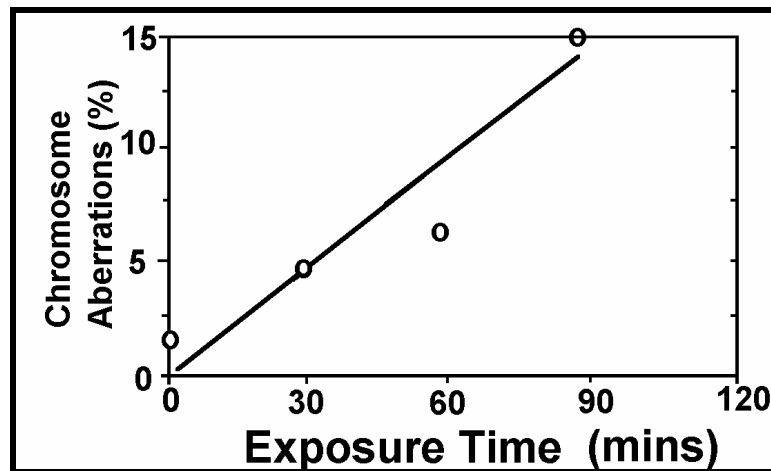
Figure 13: Chromosome aberrations in V79 Chinese hamster cells exposed to 7.7 GHz microwaves at 30 mW/cm 2 , Garaj-Vrhovac, Horvat and Koren (1991).
