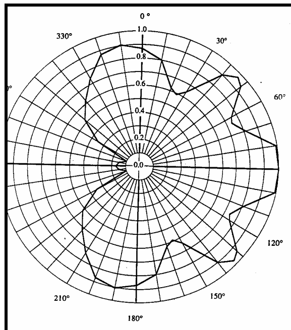
Figure 31: Horizontal antenna radiation patterns showing the relative field strength for, (a) UHF Digital TV (linear scale) from the Sutra Tower.
