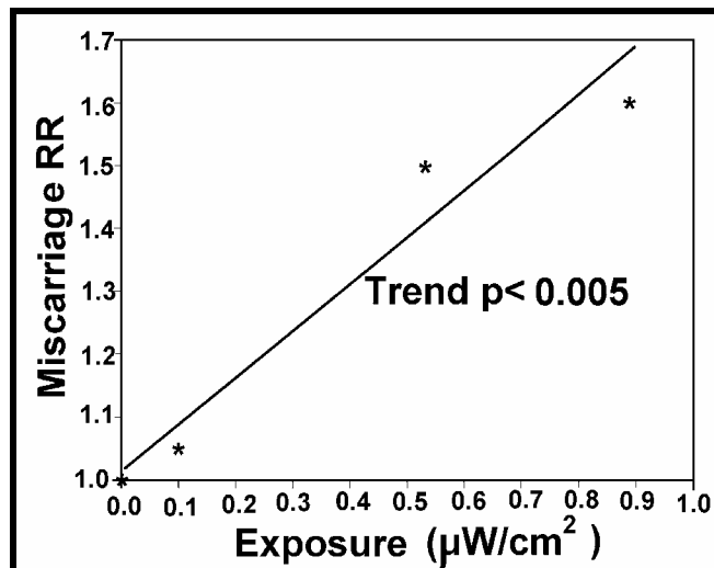
Figure 8: Microwave exposure associated first trimester miscarriage, Ouellet-Hellstrom and Stewart (1993). Exposure is monthly mean exposure based on treatments/month, 3 minutes/treatment at 600 \mu\text{W}/\text{cm}^2 .
