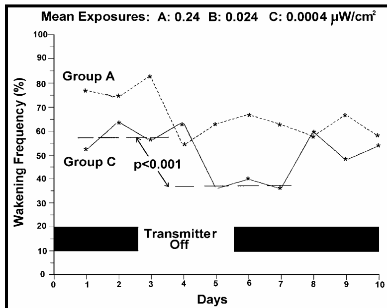
Figure 43: Sleep disturbance in people exposed to a short-wave radio stations which was turned off for three days, Altpeter et al. (1995), showing the highest exposed Group A, and lowest exposed Group C.
