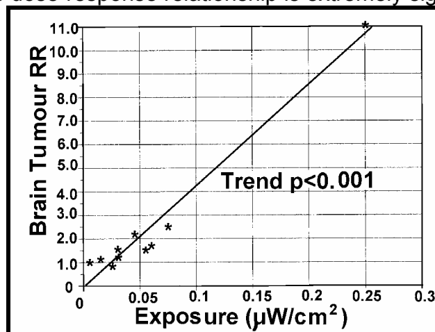
Figure 40: Brain Tumour Risk Ratio as a function of estimated radial group mean personal exposure to RF/MW radiation from the Sutra Tower, San Francisco, using the spatial childhood cancer data presented in Selvin et al. (1992). The linear dose-response relationship is extremely significant ( p < 0.001 ).
