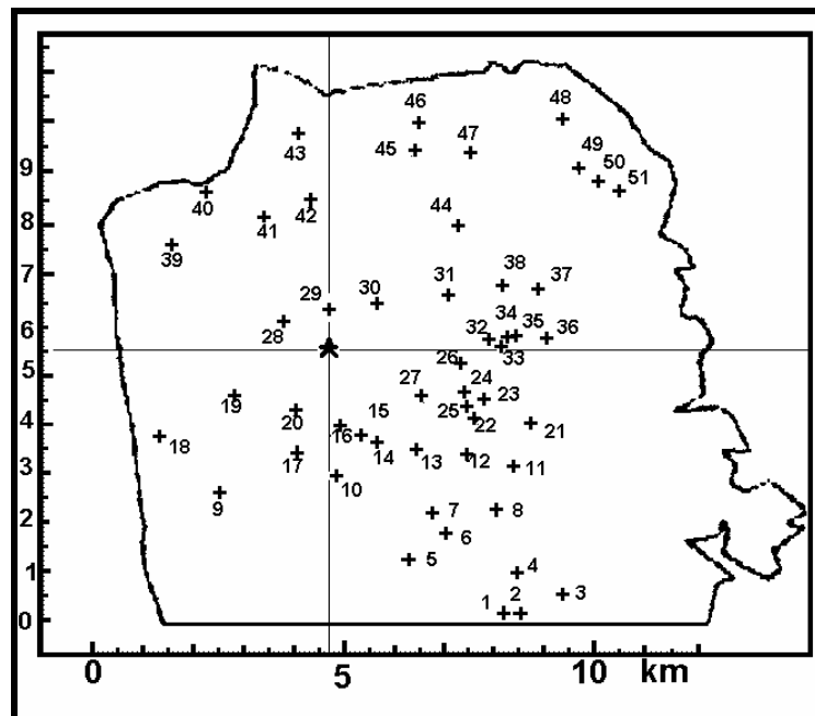
Figure 37: Spatial map of white childhood (<21 years) leukaemia for San Francisco, 1973-88, from Selvin et al. (1992).
